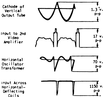
Figure 3. Typical television waveforms
